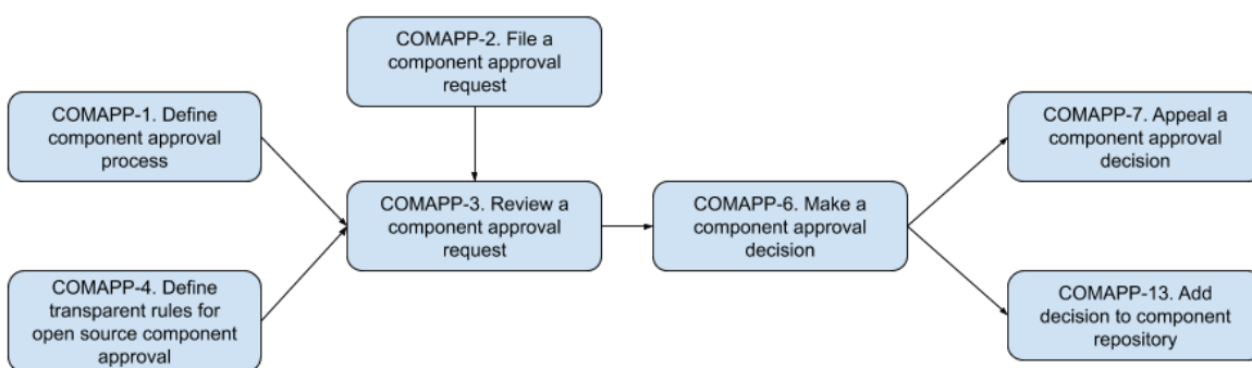
Figure 1. An example of a workflow diagram for FLOSS Governance and Component Approval - Process Template A
