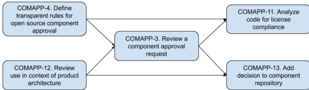
Figure 2. Another example of a workflow diagram for FLOSS Governance and Component Approval - Process Template B
